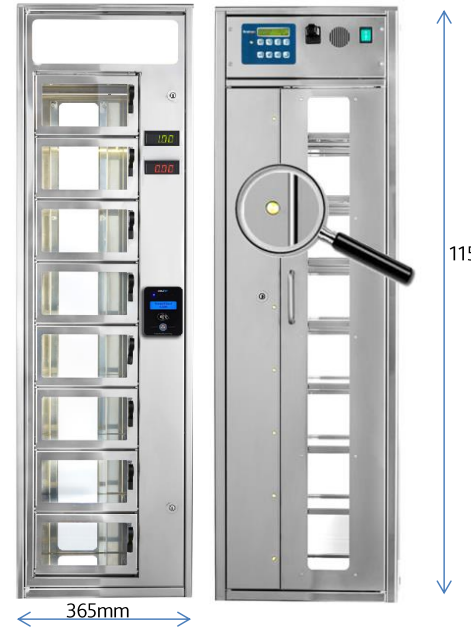
MAXI 365 front and rear view
